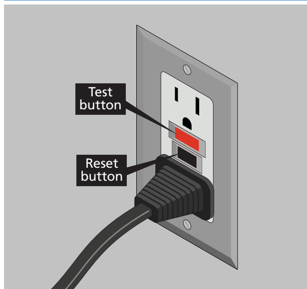
GFCI outlet
